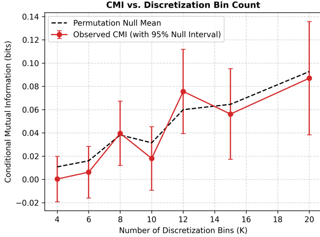
Figure 8. Conditional Mutual Information (CMI) as a function of the discretization bin count K , compared against the permutation null distribution.
