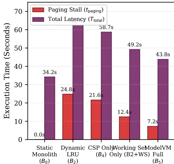
(b) Paging Stalls & Total Latency (Factor B Effect: -71% Paging Stall)
