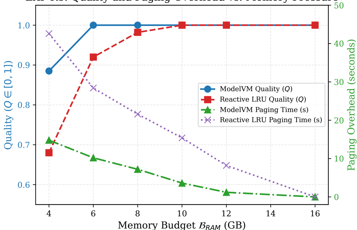
EXP-R1: Quality and Paging Overhead vs. Memory Pressure
