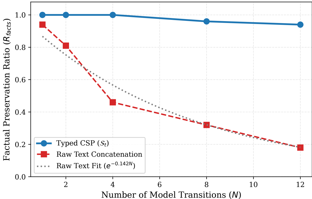
EXP-R2: State Retention vs. Model Transition Depth
