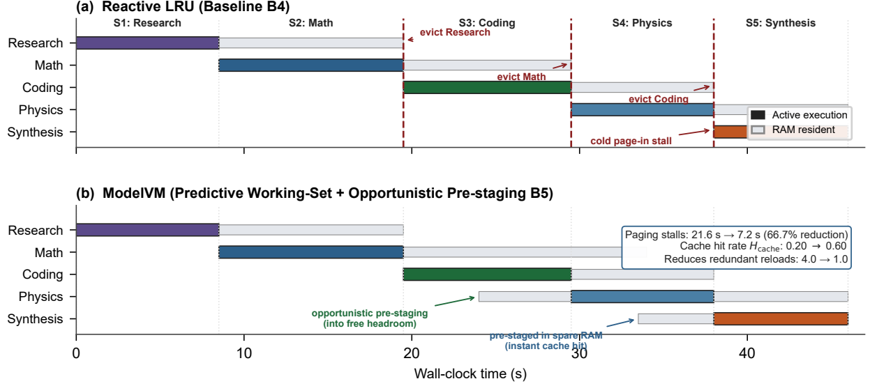
Figure 5: Working-Set Paging Execution Timeline Comparison (Class B full-width, EXP-H2). (a) Reactive LRU ( B_4 ): Devoid of forward visibility, LRU evicts inactive models when memory headroom tightens, triggering recurrent reload stalls ( t_{\text{paging}} = 21.60 s total) and model thrashing. (b) ModelVM ( B_5 ): Combining stage-level working-set forecasting W(t, k) with cost-aware eviction shielding ( \delta \times 1.8 ) and opportunistic prefetching reduces redundant reloads (from 4.0 to 1.0), cutting paging stalls by 66.7% ( 21.60 s \rightarrow 7.20 s) and lifting cache hit rate from 0.20 to 0.60.
