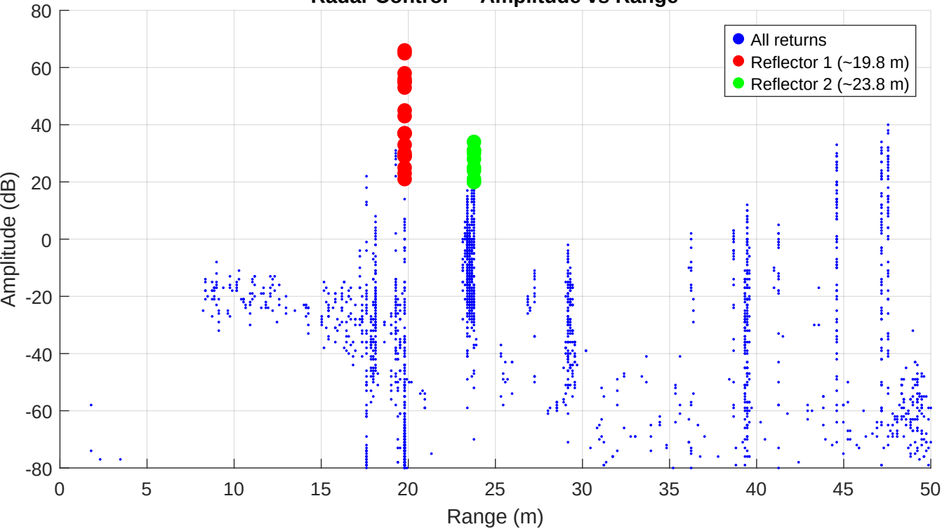
Radar Control — Amplitude vs Range
