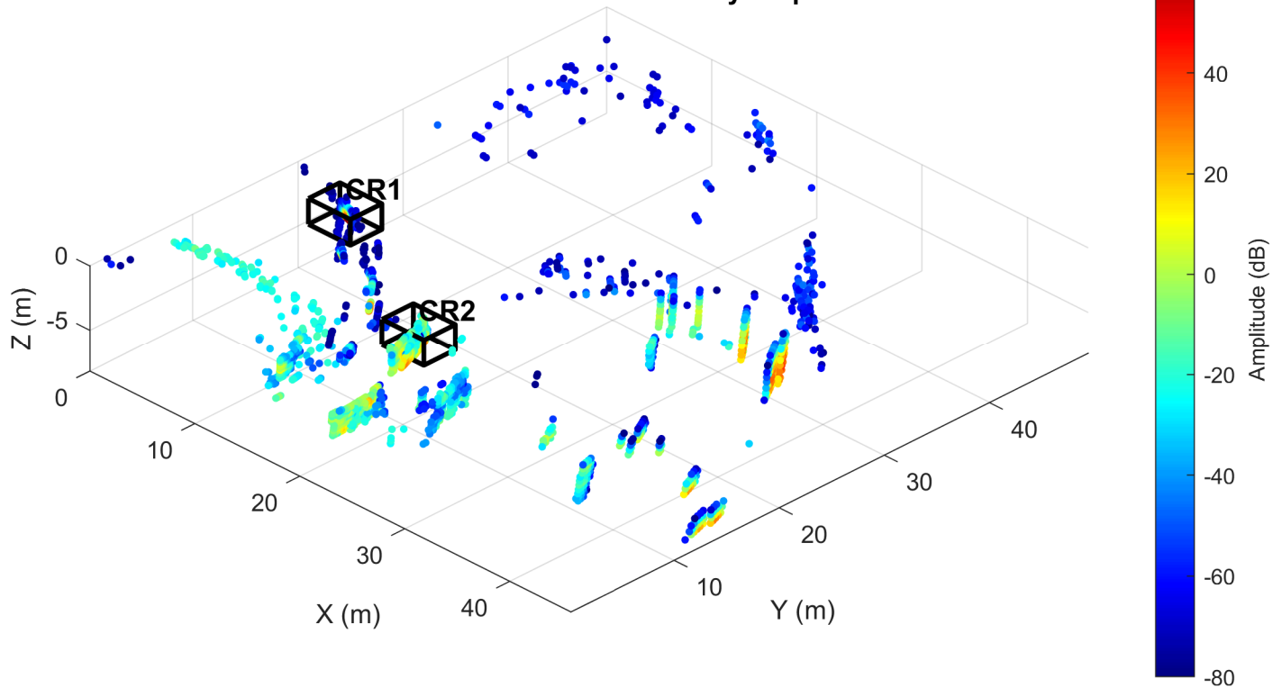
Radar Control Scan — Coloured by Amplitude
