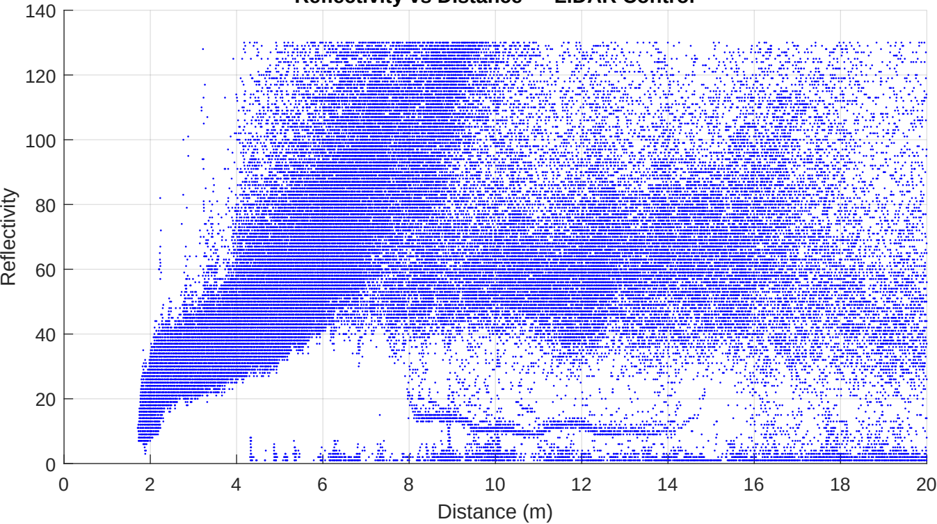
Reflectivity vs Distance — LiDAR Control
