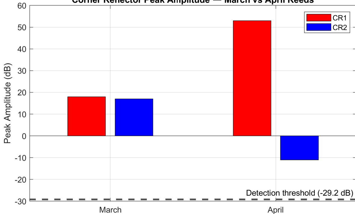
Corner Reflector Peak Amplitude — March vs April Reeds
