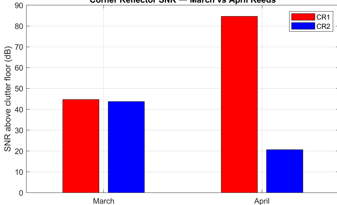
Corner Reflector SNR — March vs April Reeds
