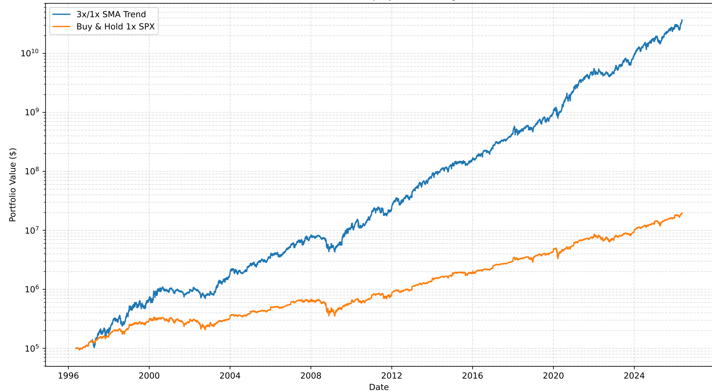
S&P 500 Backtest: Equity Curves (Log Scale)
