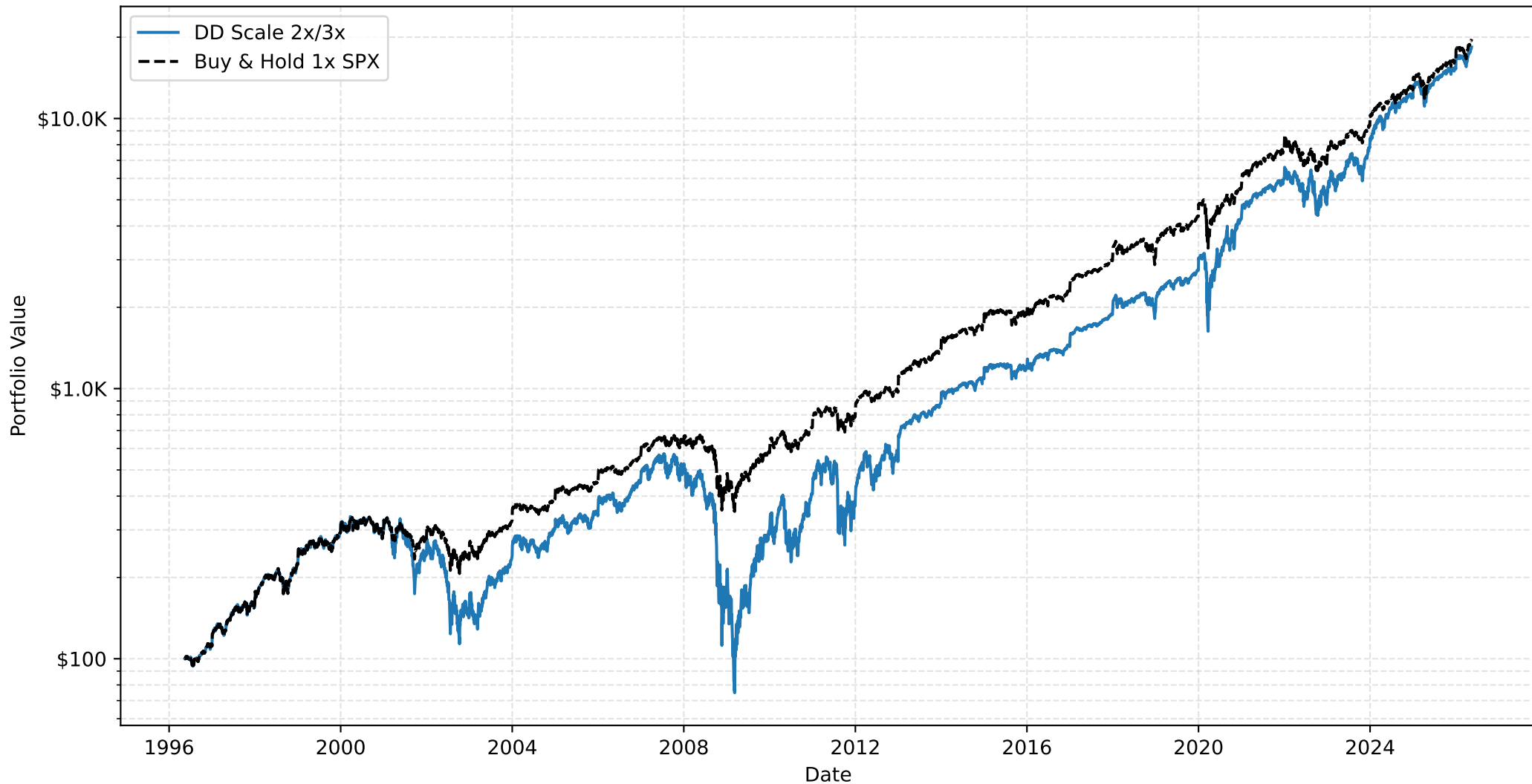
DD Scale 2x/3x vs Buy & Hold 1x SPX
