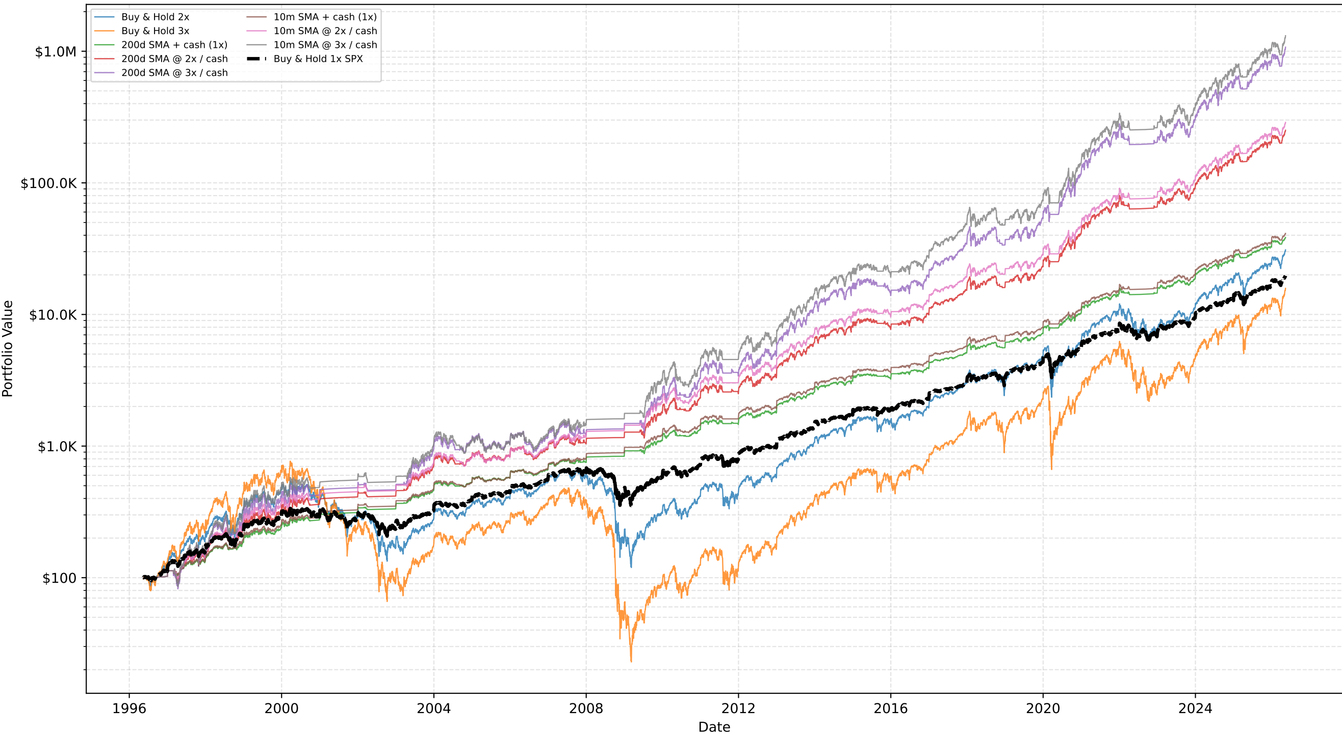
SMA Trend & Buy & Hold: 1x / 2x / 3x
