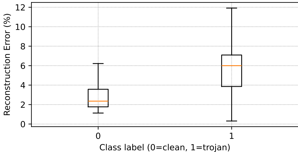
Reconstruction Error per Class Type (Trojan Detection)
