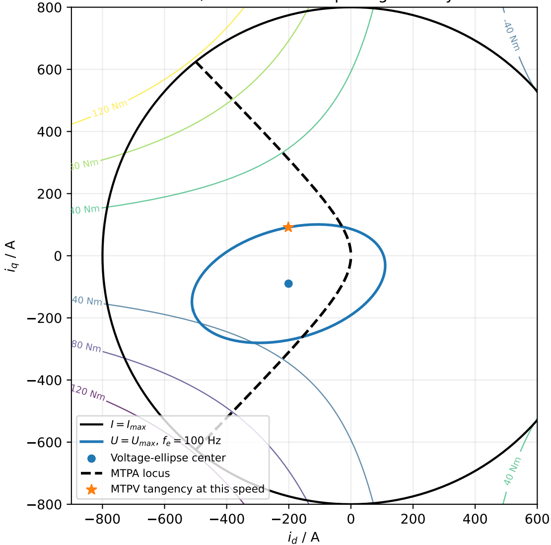
PMSM/IPMSM current-space geometry
