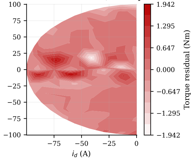
Corrected centered residual, 3000 rpm
