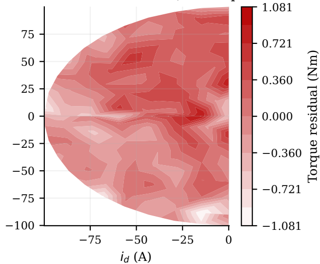
Corrected centered residual, 1000 rpm
