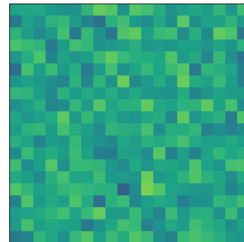
Shifted rastrigin vs rank (matched d per method)
