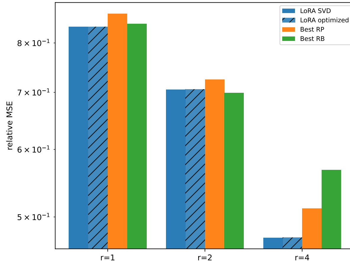
Reconstruction error vs LoRA rank
