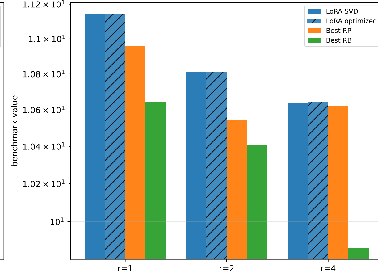
Shifted rastrigin objective vs LoRA rank
