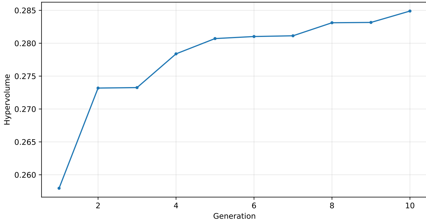
Hypervolume per generation (final 0.2849)
