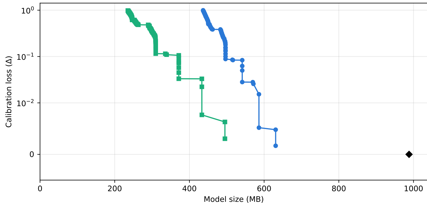
Qwen2.5-0.5B: final Pareto fronts ( \Delta \leq 1 )
