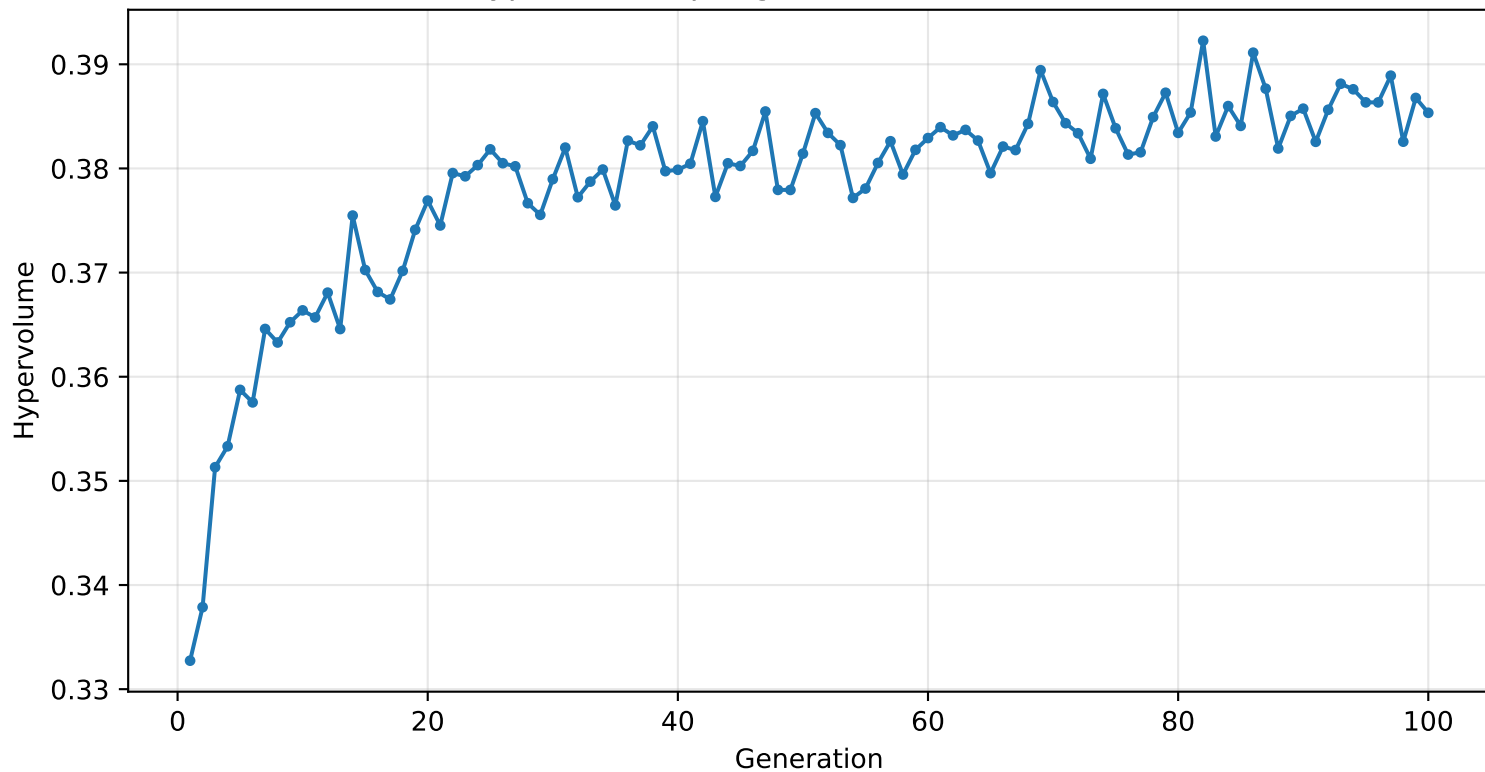
Hypervolume per generation (final 0.3853)
