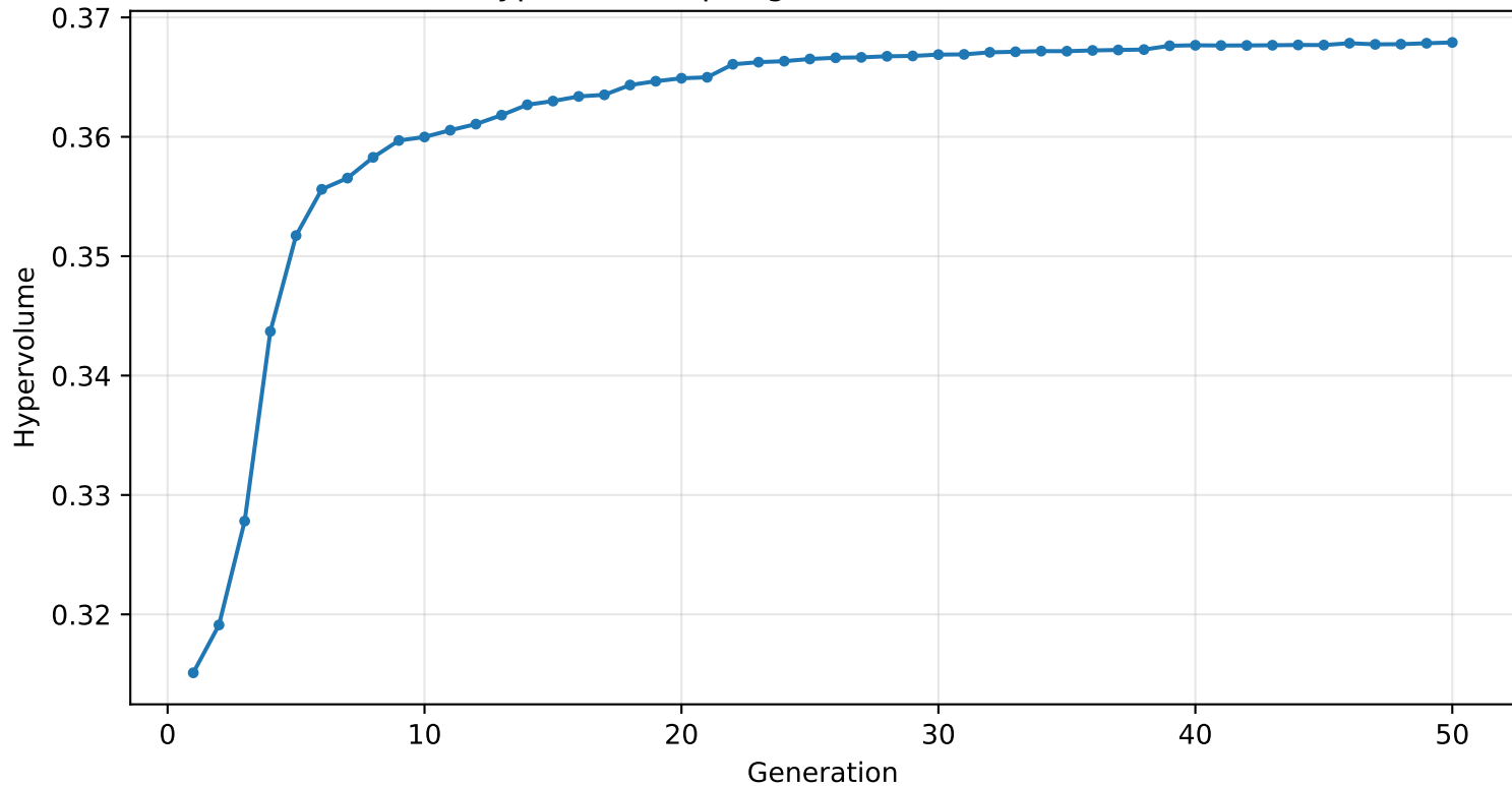
Hypervolume per generation (final 0.3679)
