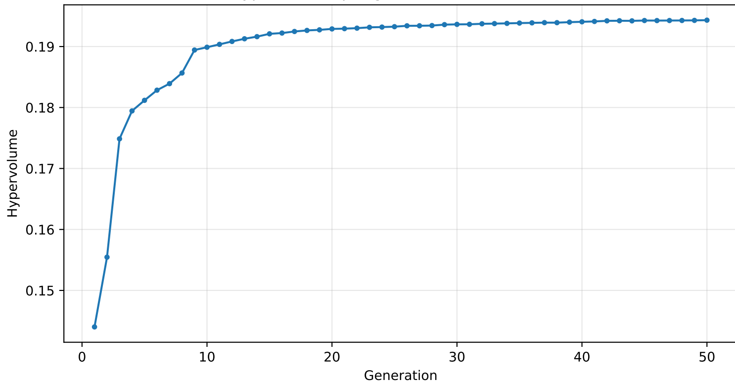
Hypervolume per generation (final 0.1943)
