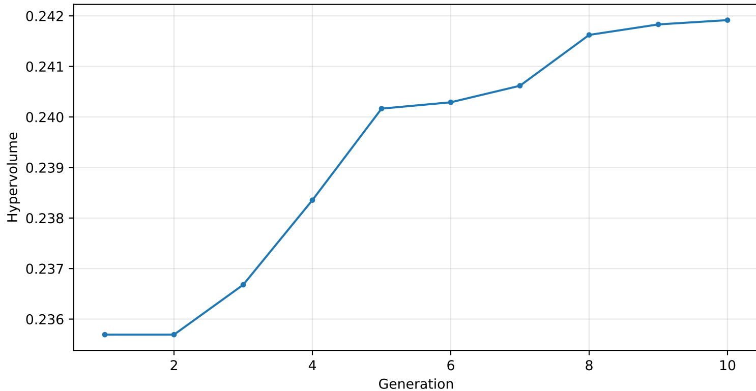
Hypervolume per generation (final 0.2419)
