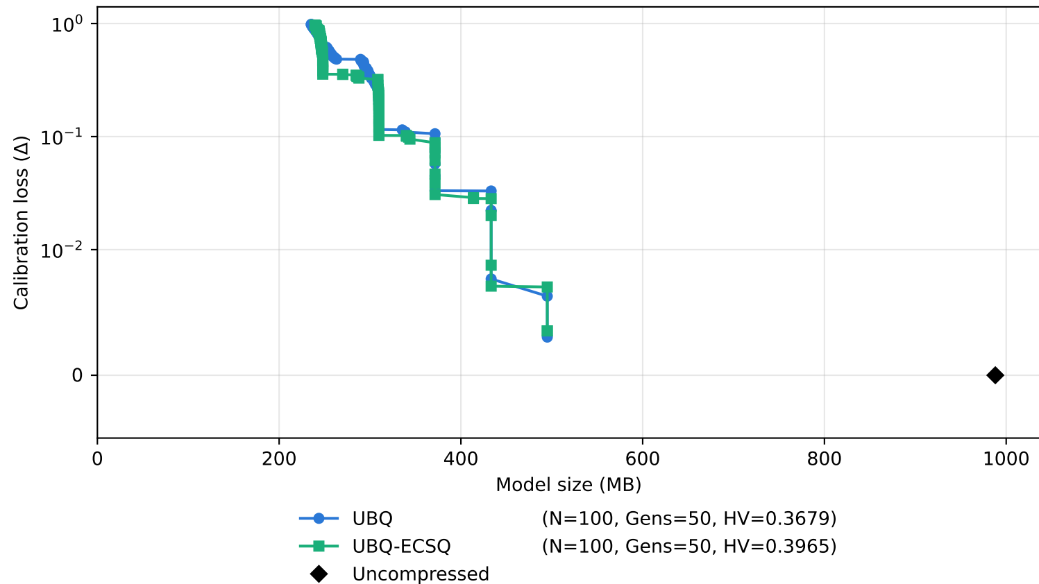
Qwen2.5-0.5B, Linear layers + Embedding: final Pareto fronts ( \Delta \leq 1 )
