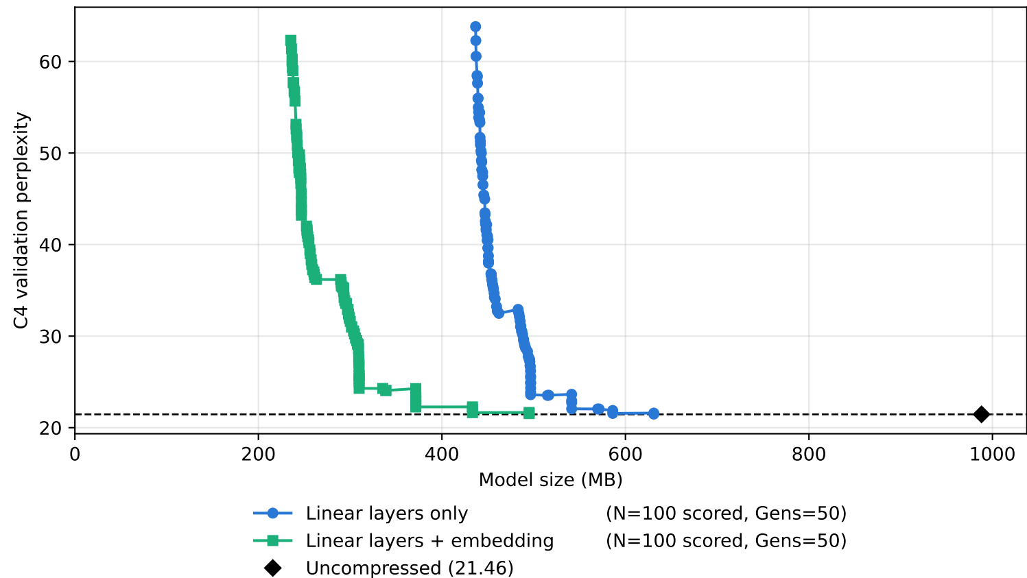
Qwen2.5-0.5B, UHQ
