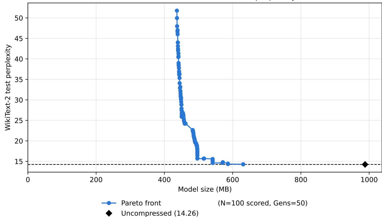
Final Pareto fronts: WikiText-2 test perplexity
