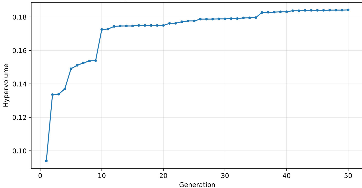
Hypervolume per generation (final 0.1843)
