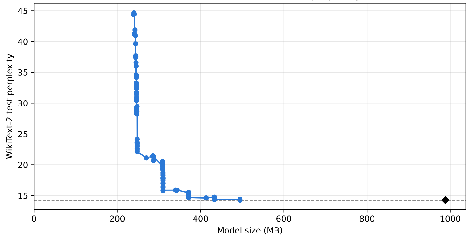
Final Pareto fronts: WikiText-2 test perplexity
