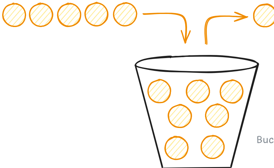
Token Bucket
