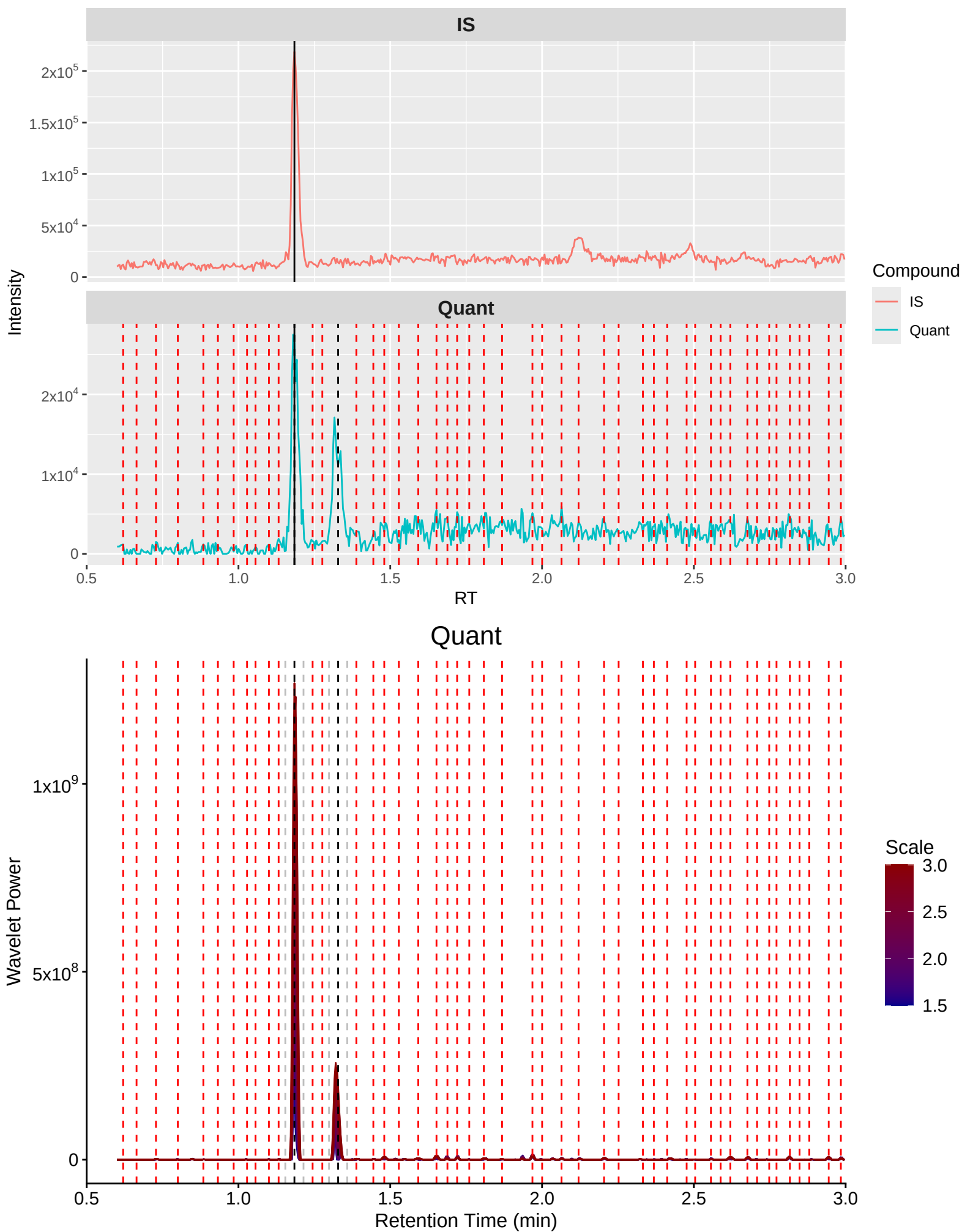
Gabapentin Quant (m/z 172.3 → 154.3): 16X 3 (waters)
