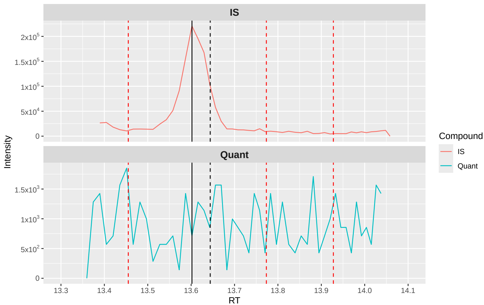
RvT4 Quant (m/z 361.1 \rightarrow 211.1): WD 1 (6500)
