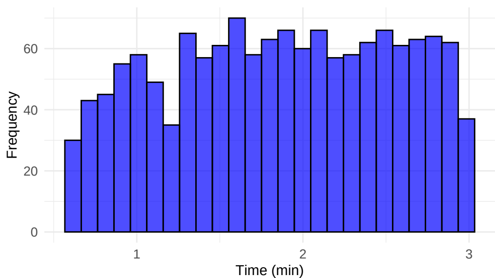
(e) Gabapentin Quant (m/z 172.3 \rightarrow 154.3)
