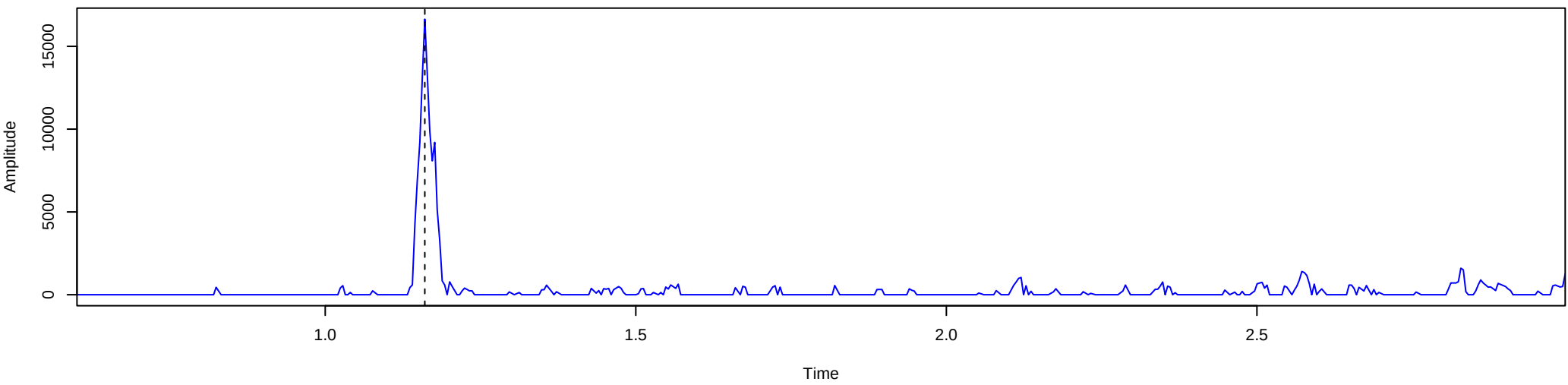
Mexican Hat Wavelet Power Spectrum (asinh scaled)
