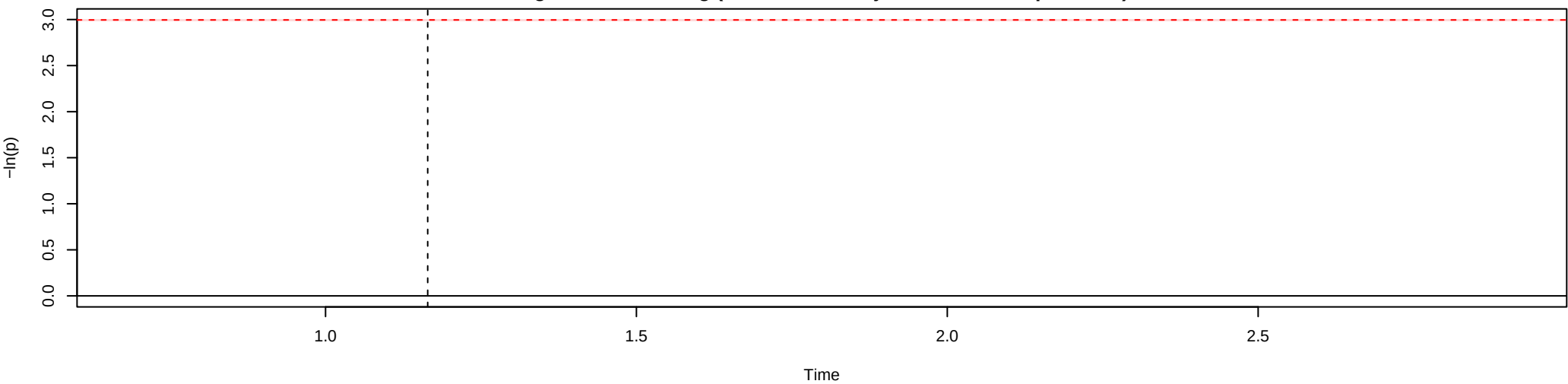
Significance Testing (Holm FWER-adjusted minimum p-values)
