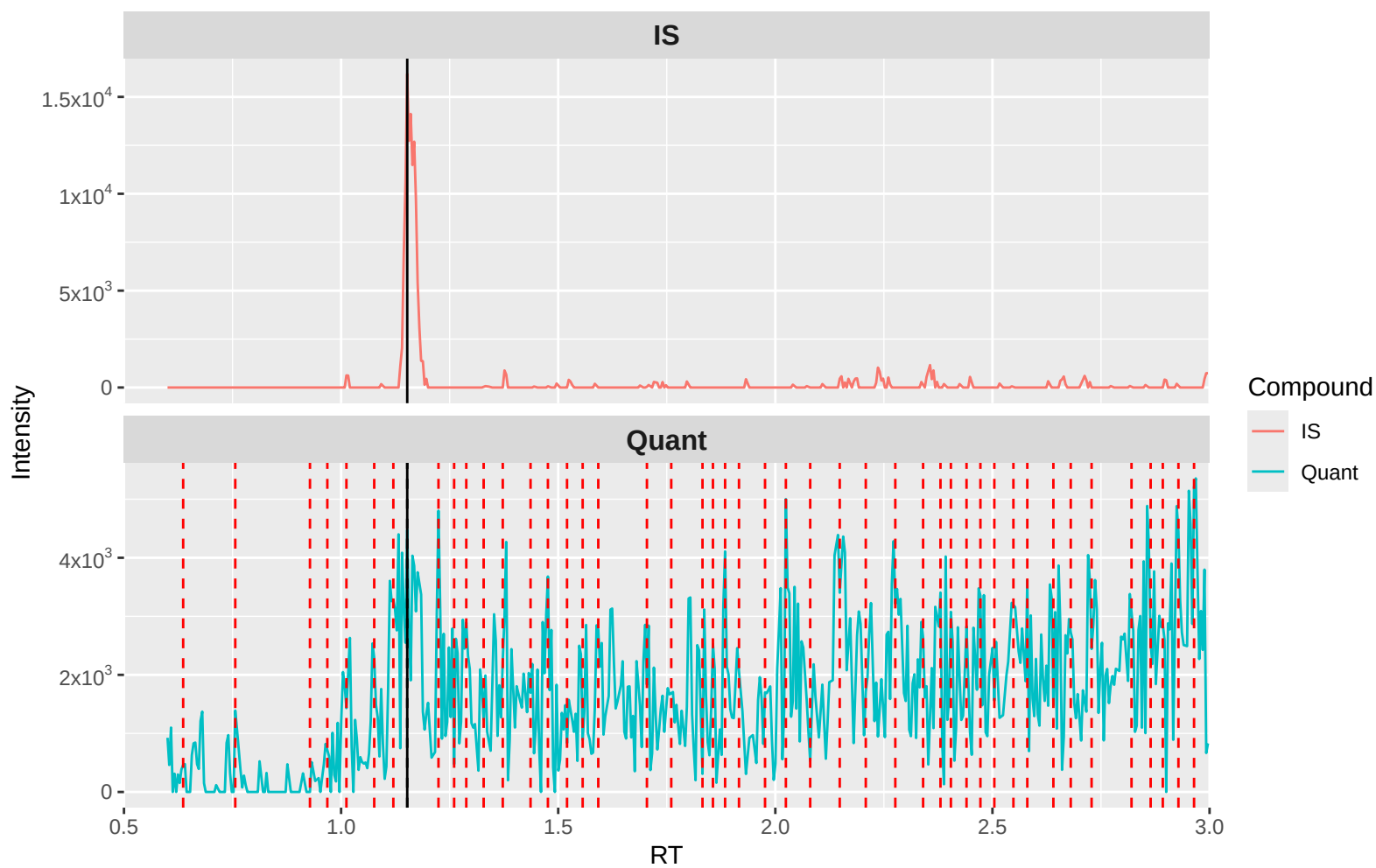
Clonidine Quant (m/z 232.2 → 215.1): 0_5X 1 (waters)
