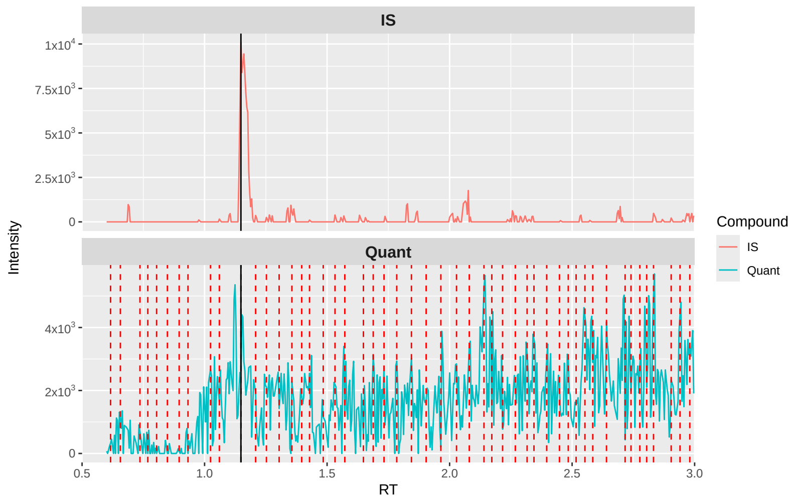
Clonidine Quant (m/z 232.2 → 215.1): 0_25X 3 (waters)
