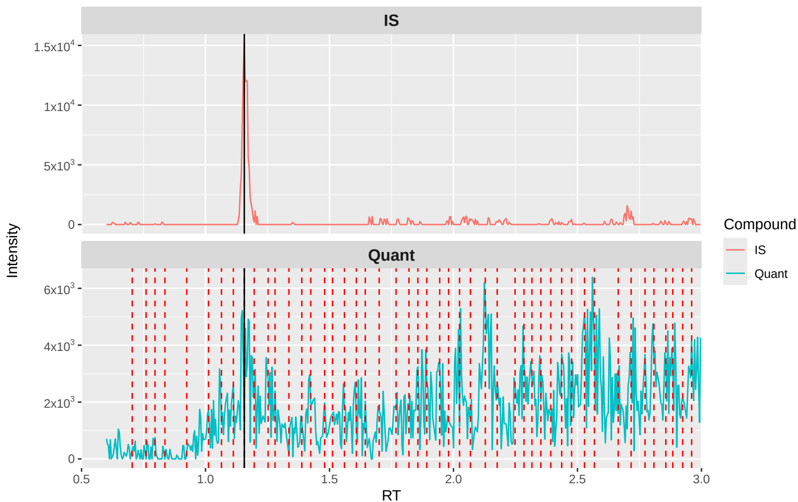
Clonidine Quant (m/z 232.2 → 215.1): 0_25X 1 (waters)
