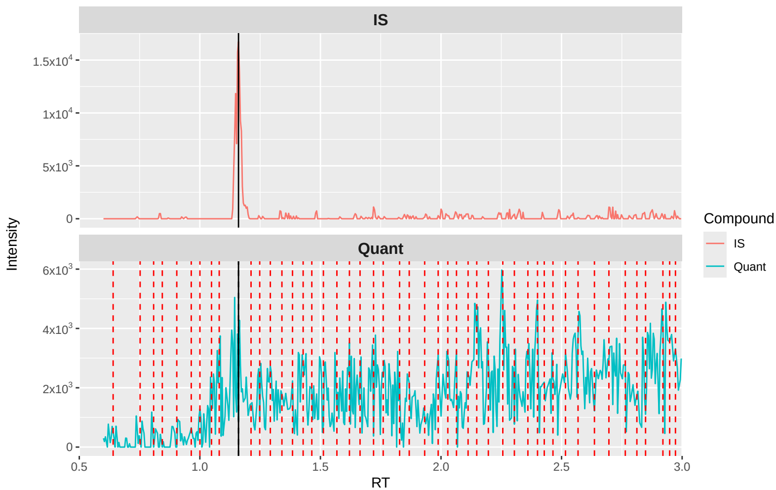
Clonidine Quant (m/z 232.2 → 215.1): Blank 1 (waters)
