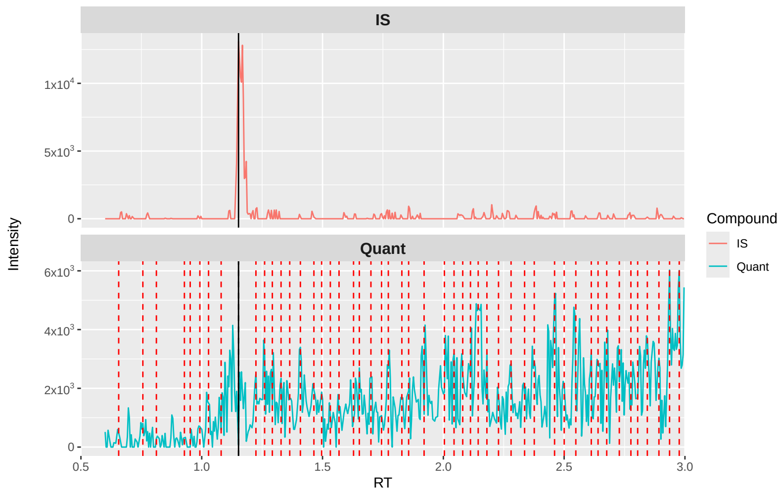
Clonidine Quant (m/z 232.2 → 215.1): 0_25X 2 (waters)
