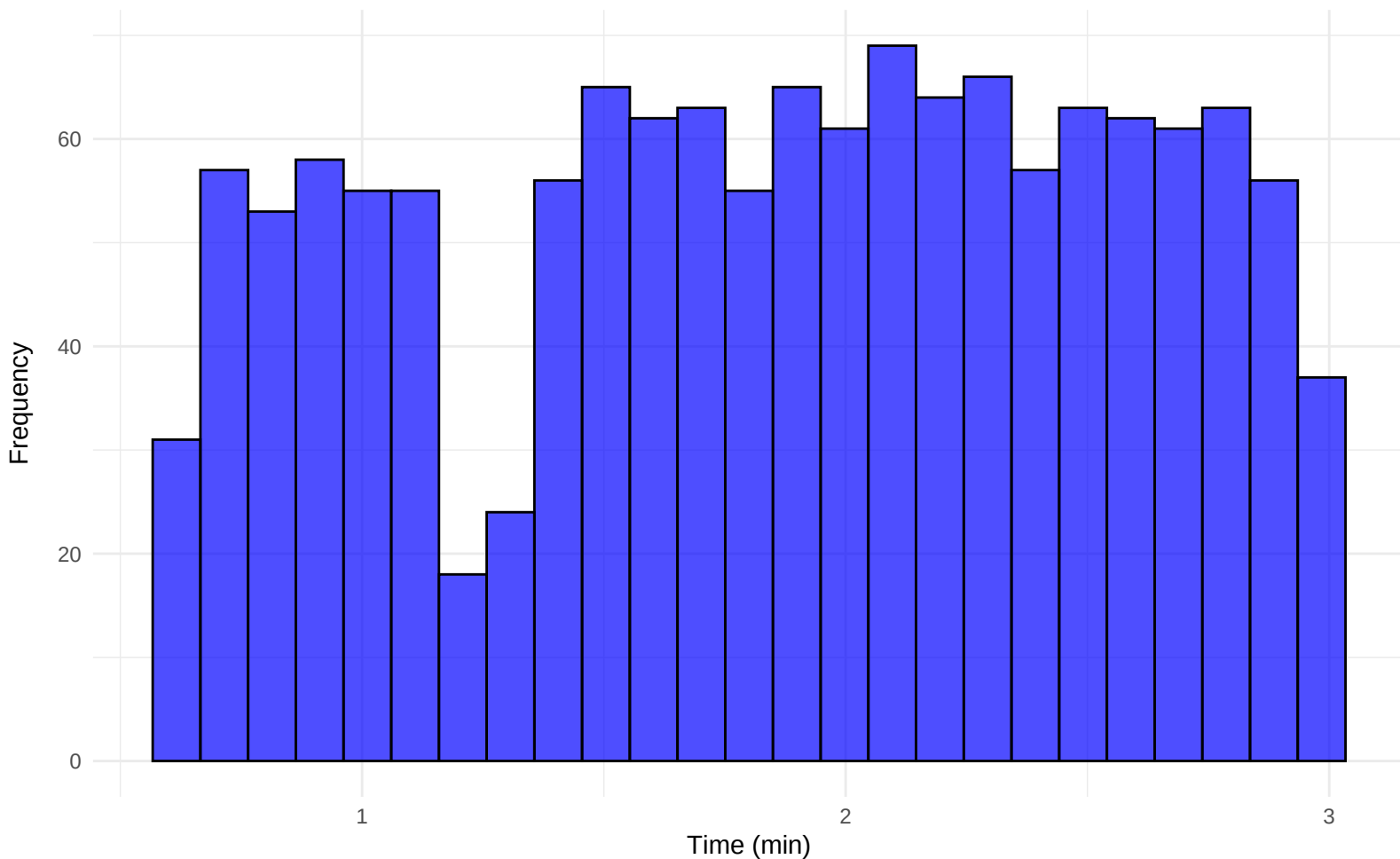
Peak Power Distribution – Gabapentin Quant (m/z 172.3 → 154.3) – waters
