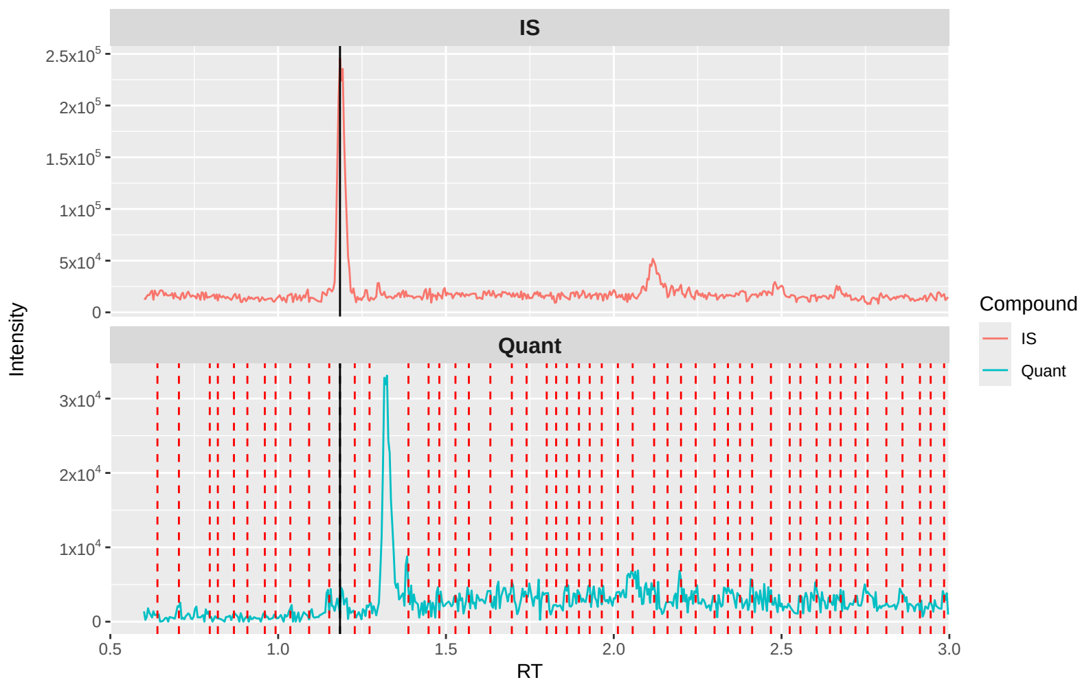
Gabapentin Quant (m/z 172.3 → 154.3): 0_5X 1 (waters)
