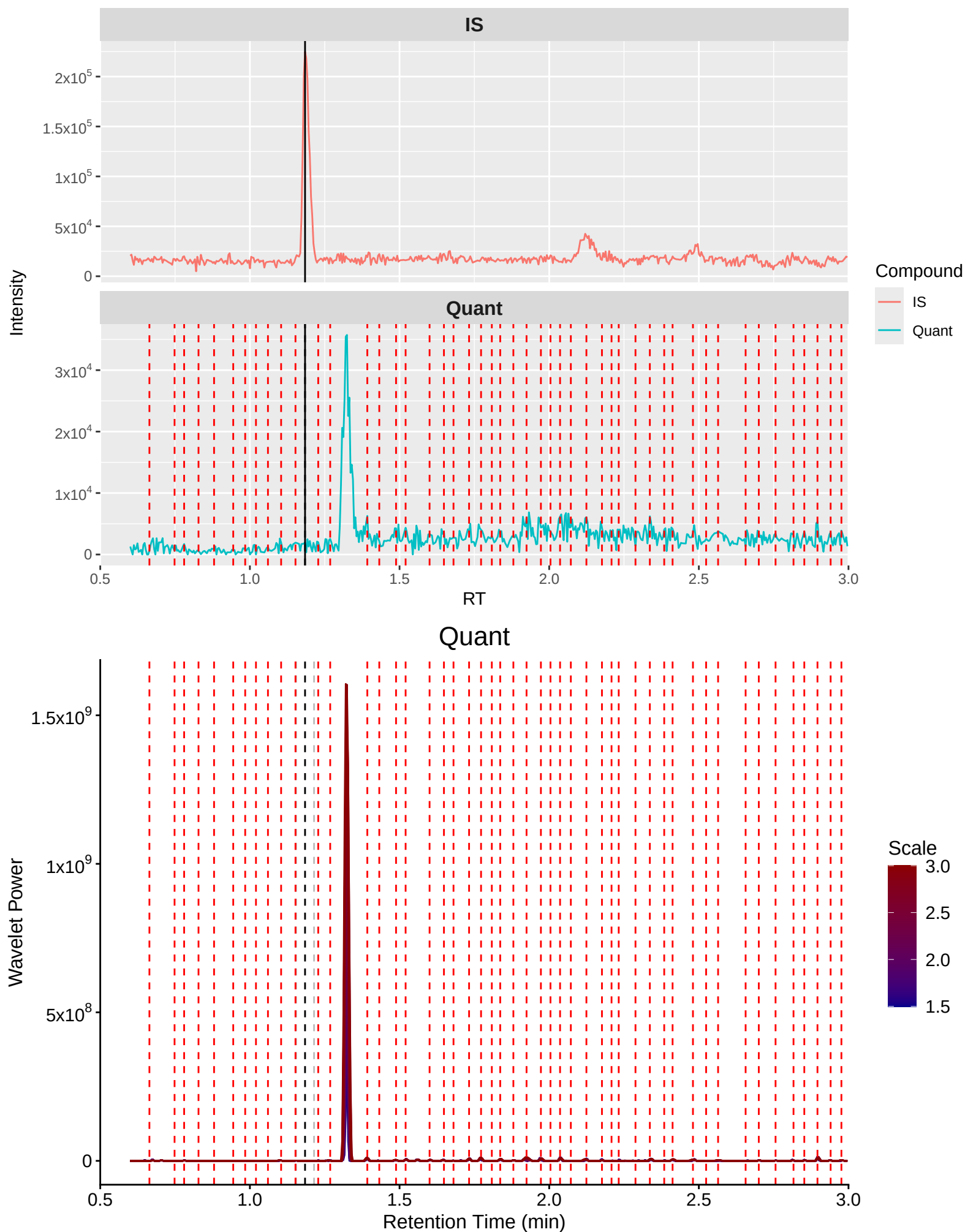
Gabapentin Quant (m/z 172.3 → 154.3): 0_25X 3 (waters)
