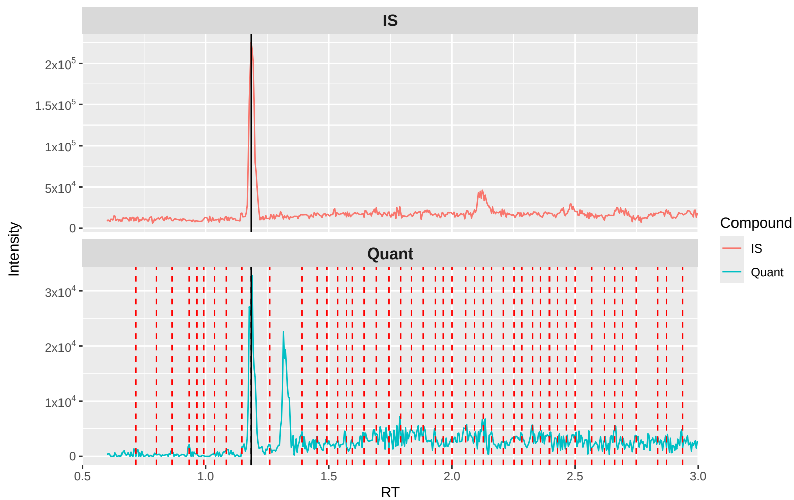
Gabapentin Quant (m/z 172.3 → 154.3): 16X 2 (waters)
