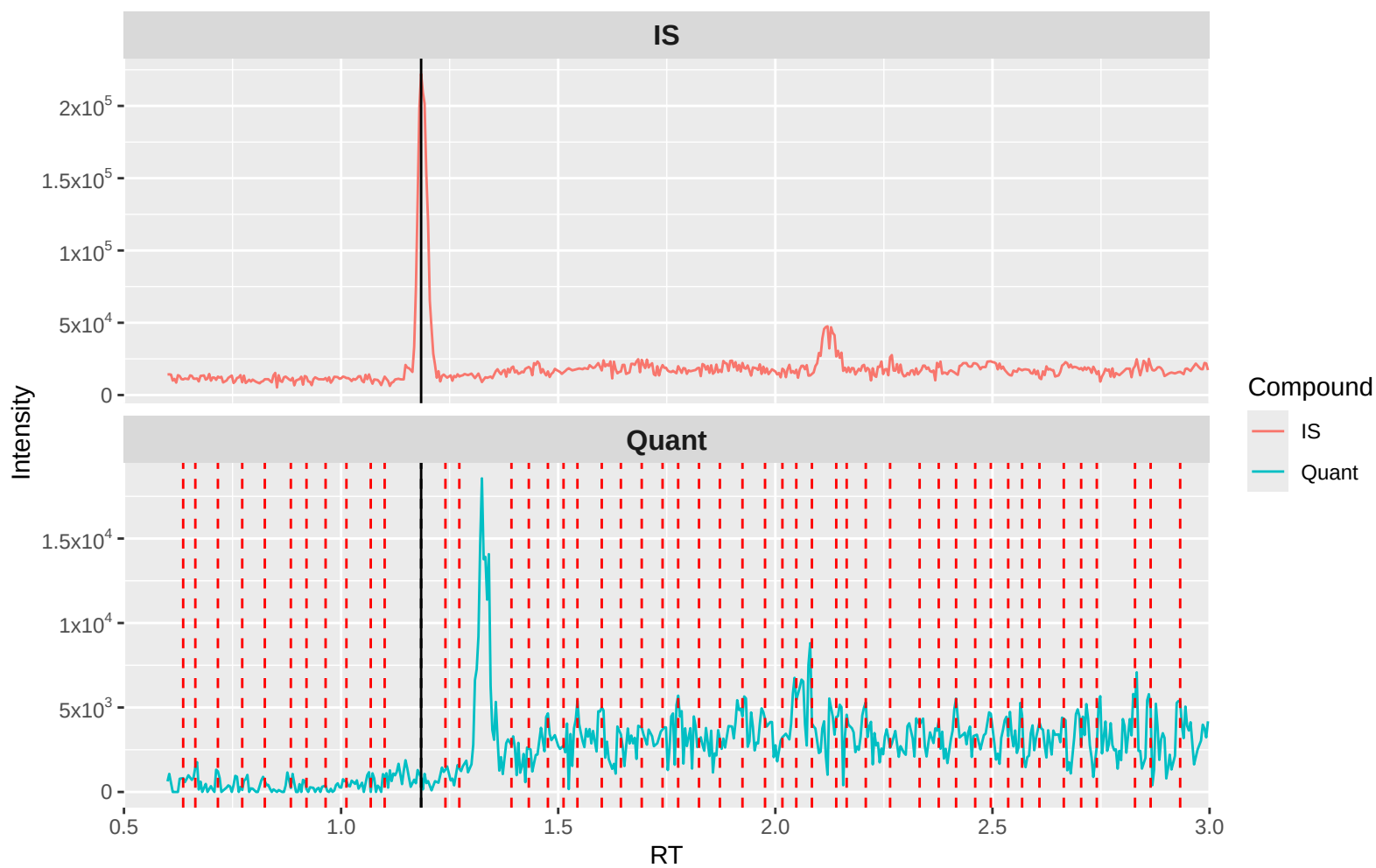
Gabapentin Quant (m/z 172.3 → 154.3): Blank 1 (waters)
