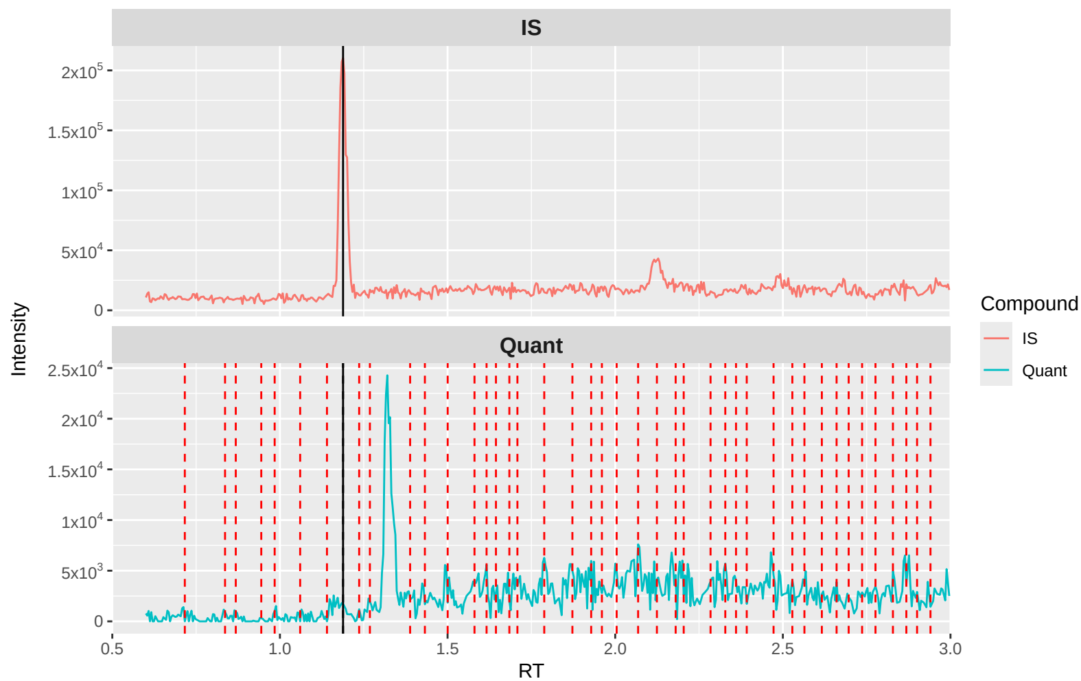
Gabapentin Quant (m/z 172.3 → 154.3): 1X 3 (waters)
