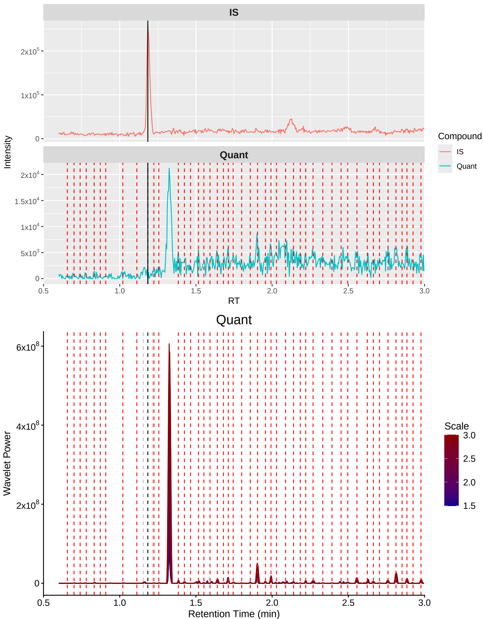
Gabapentin Quant (m/z 172.3 → 154.3): Blank 3 (waters)
