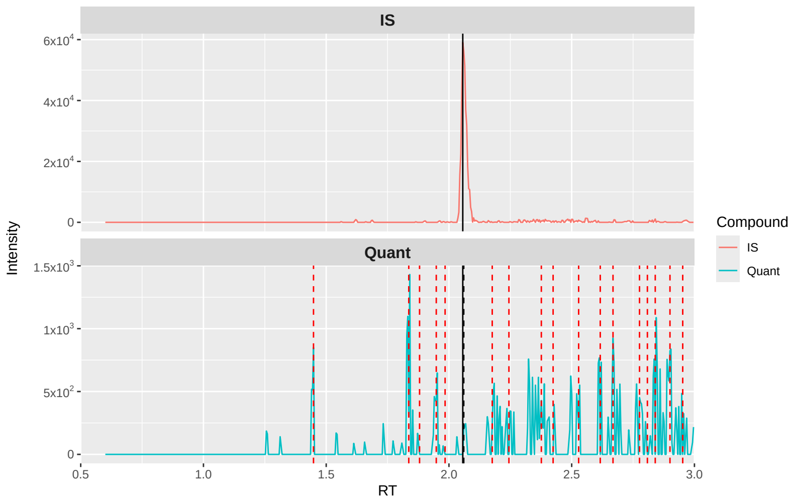
Lorazepam Quant (m/z 321.2 \rightarrow 275): Blank 3 (waters)
