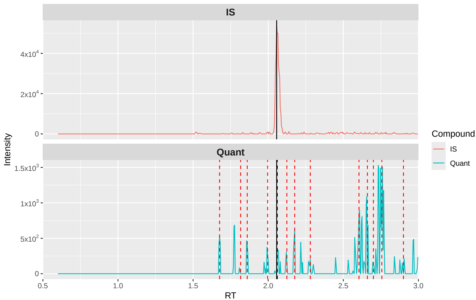
Lorazepam Quant (m/z 321.2 → 275): Blank 2 (waters)
