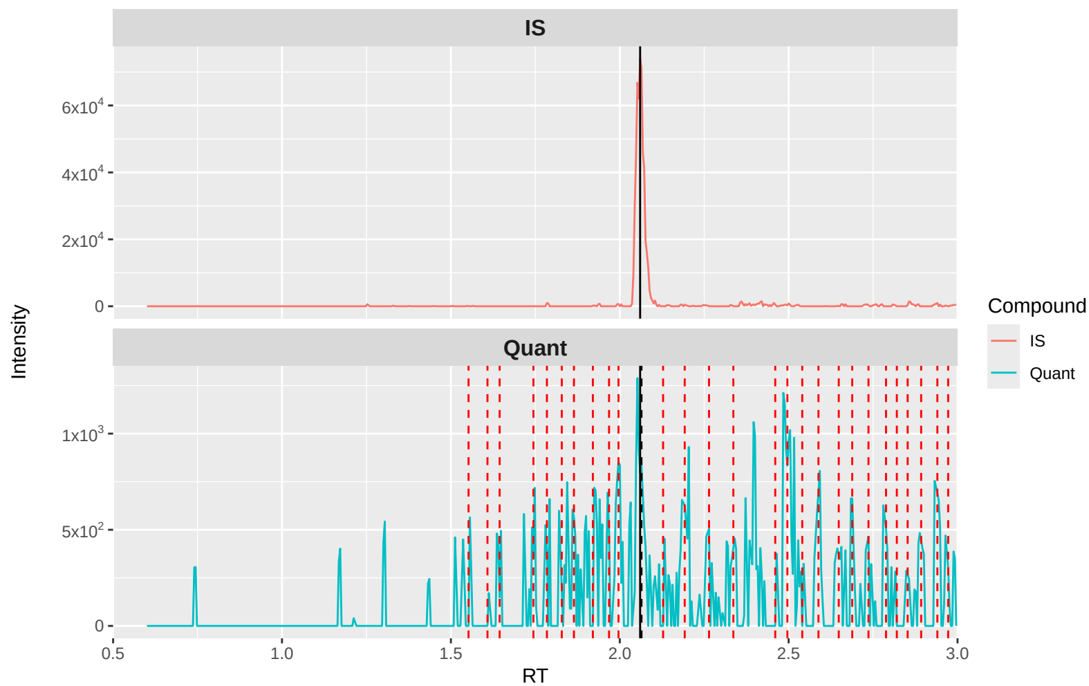
Lorazepam Quant (m/z 321.2 \rightarrow 275): 0_5X 3 (waters)
