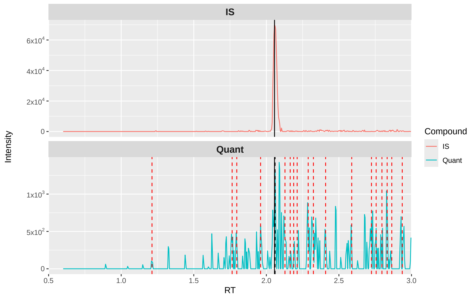
Lorazepam Quant (m/z 321.2 \rightarrow 275): 0_5X 1 (waters)
