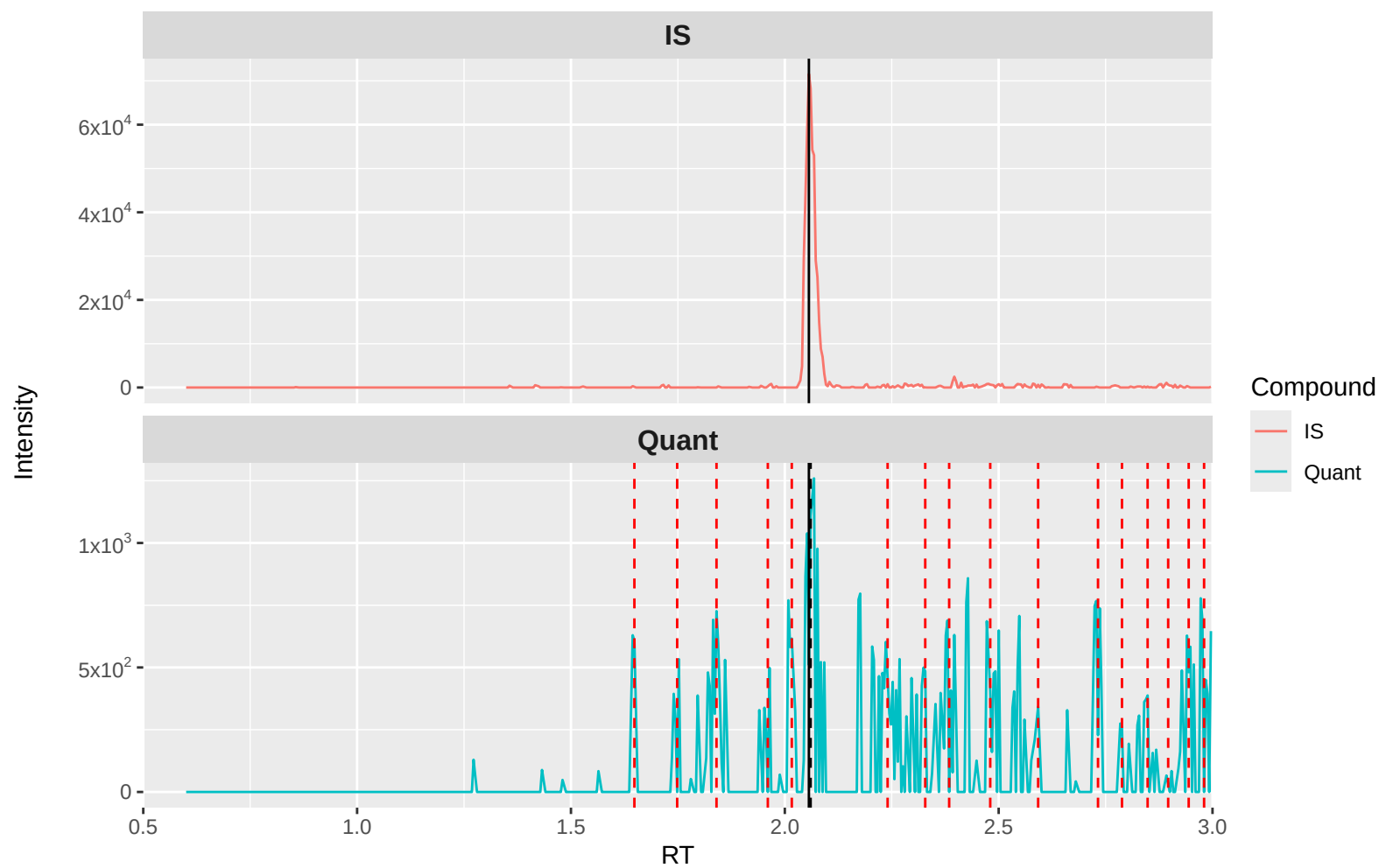
Lorazepam Quant (m/z 321.2 \rightarrow 275): 0_25X 2 (waters)
