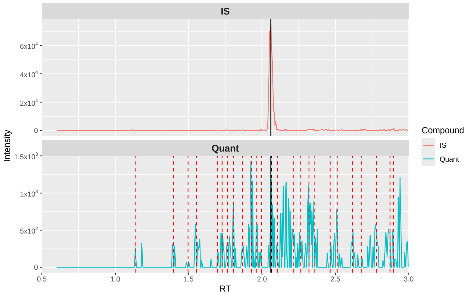
Lorazepam Quant (m/z 321.2 \rightarrow 275): 0_25X 1 (waters)
