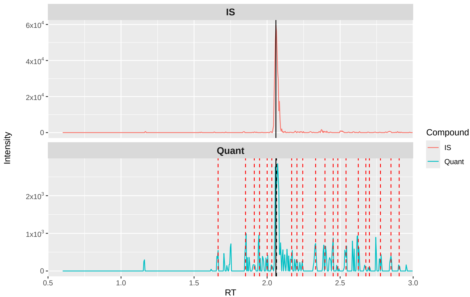
Lorazepam Quant (m/z 321.2 → 275): 2X 2 (waters)
