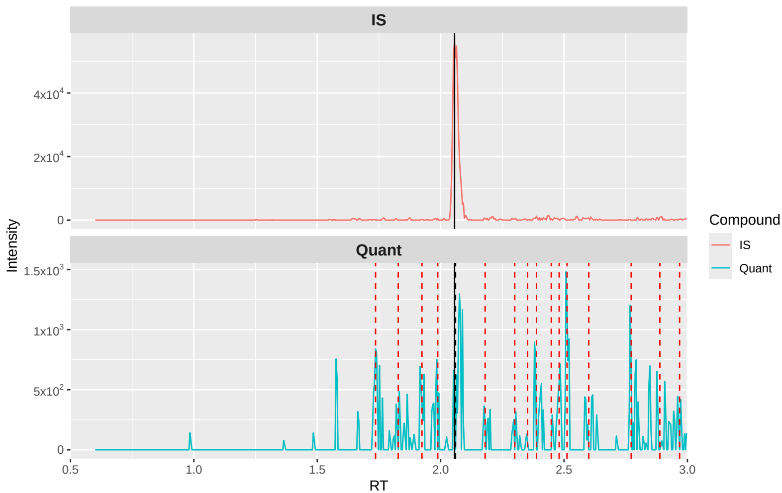
Lorazepam Quant (m/z 321.2 → 275): Blank 1 (waters)
