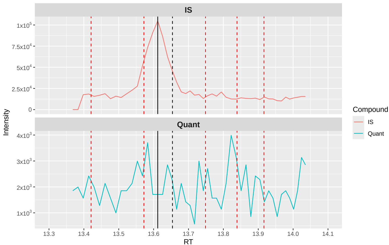
RvT4 Quant (m/z 361.1 \rightarrow 211.1): Chow 3 (6500)
