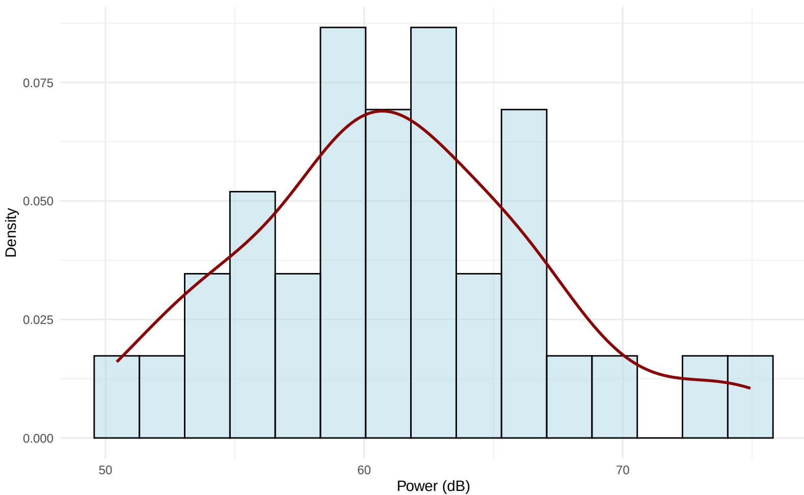
Peak Power Distribution – RvT4 Quant (m/z 361.1 → 211.1 ) – 6500
