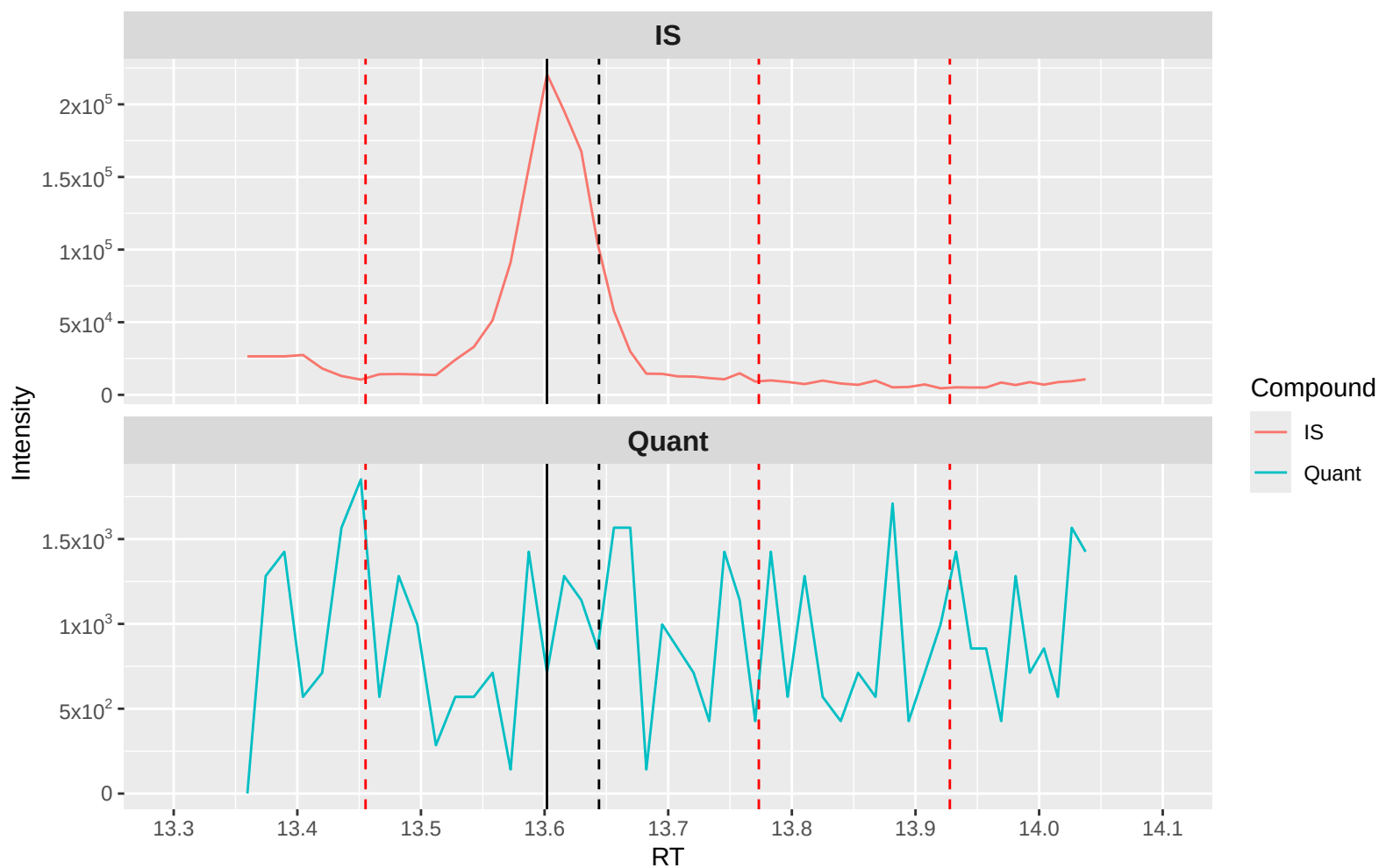
RvT4 Quant (m/z 361.1 → 211.1): WD 1 (6500)
