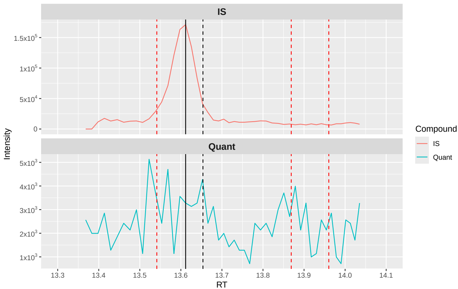
RvT4 Quant (m/z 361.1 → 211.1): Chow 1 (6500)
