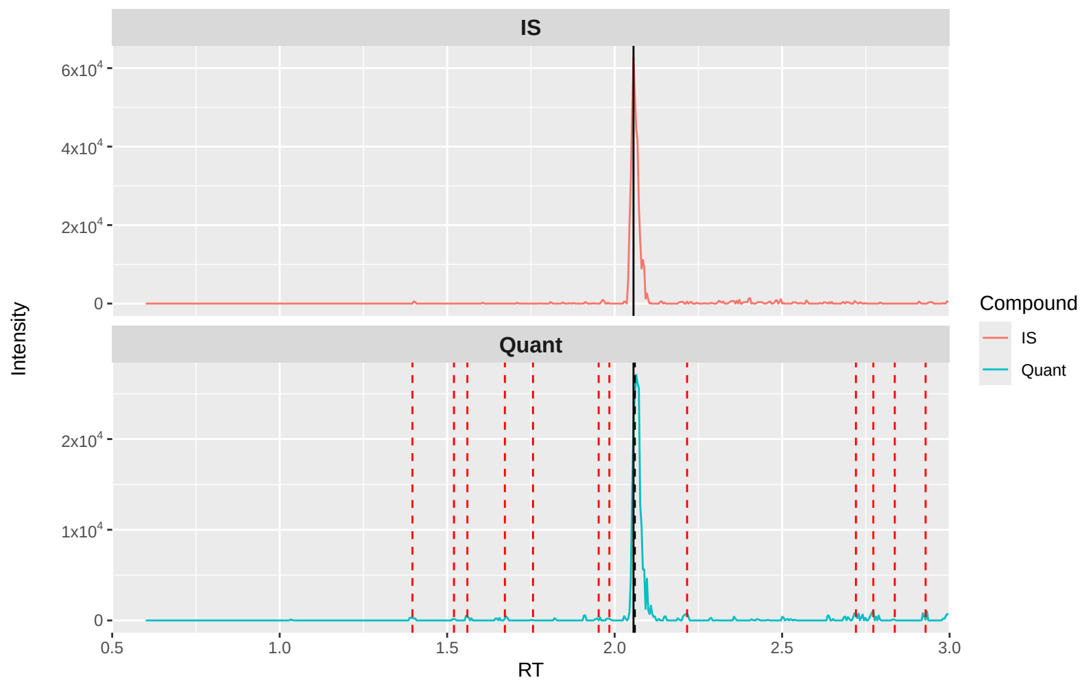
Lorazepam Quant (m/z 321.2 → 275): 16X 2 (waters)
