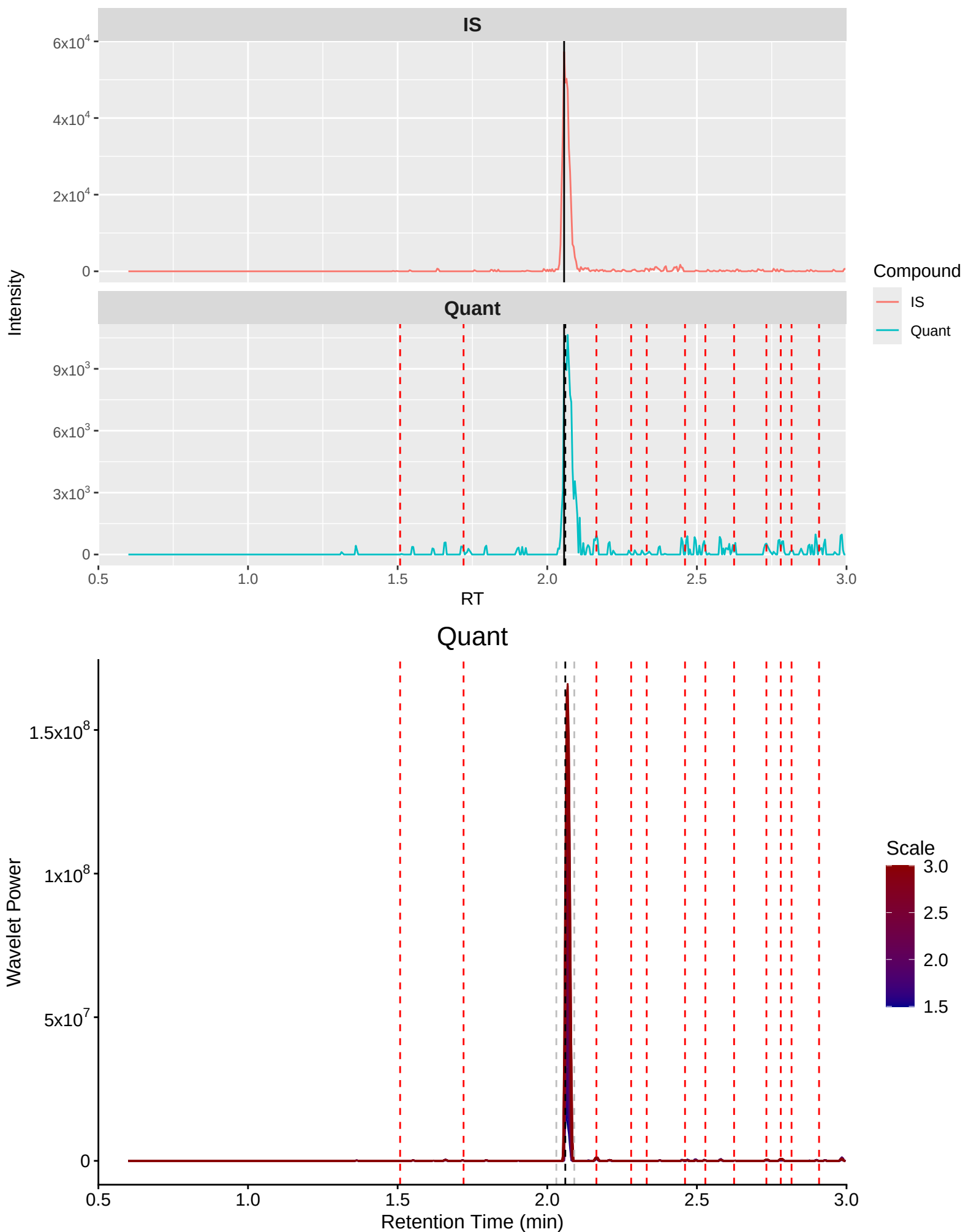
Lorazepam Quant (m/z 321.2 \rightarrow 275): 8X 3 (waters)
