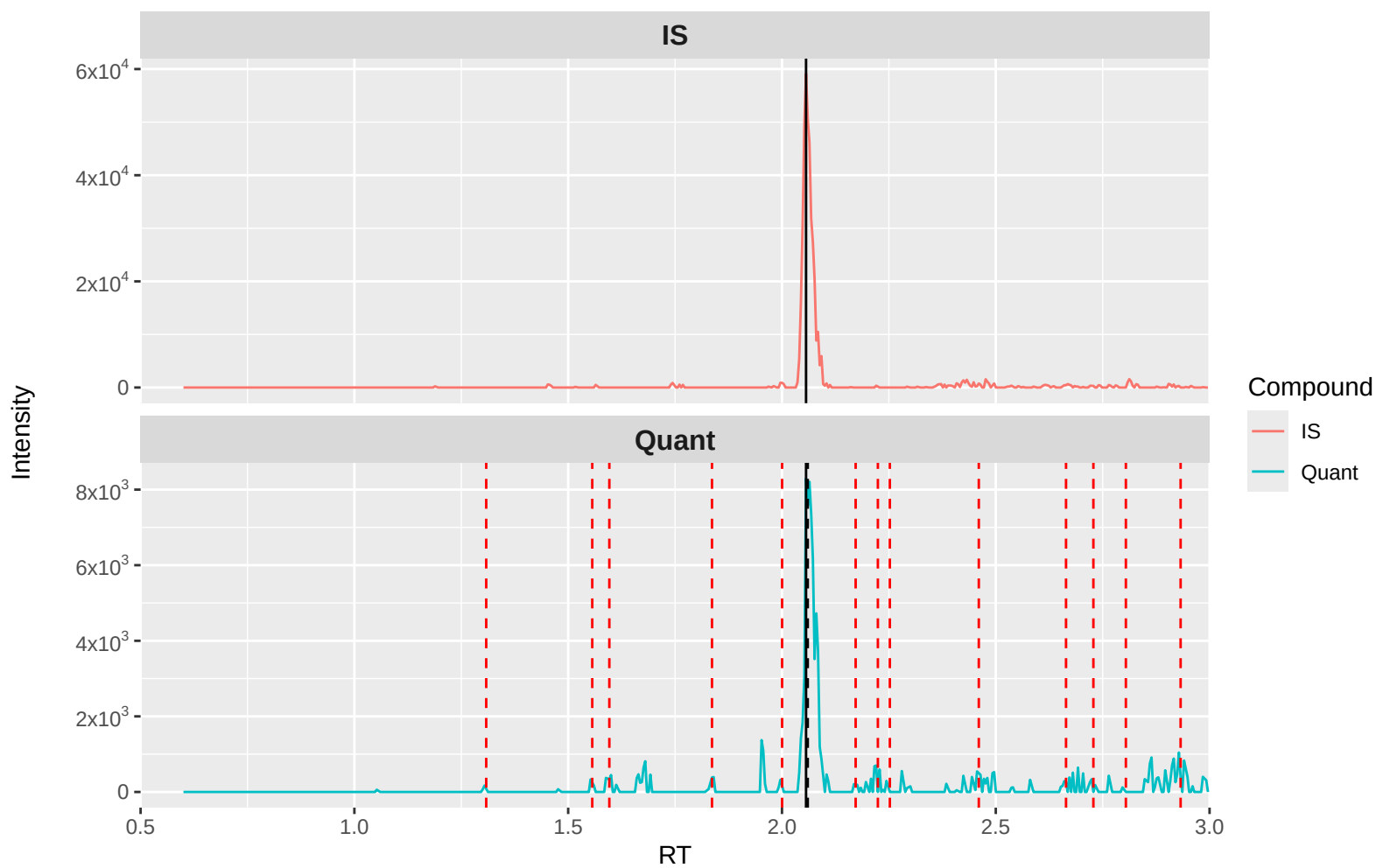
Lorazepam Quant (m/z 321.2 → 275): 4X 2 (waters)
