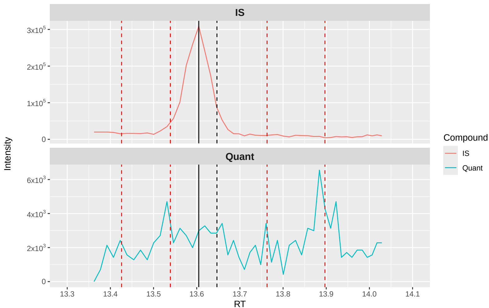
RvT4 Quant (m/z 361.1 \rightarrow 211.1): WD 3 (6500)
