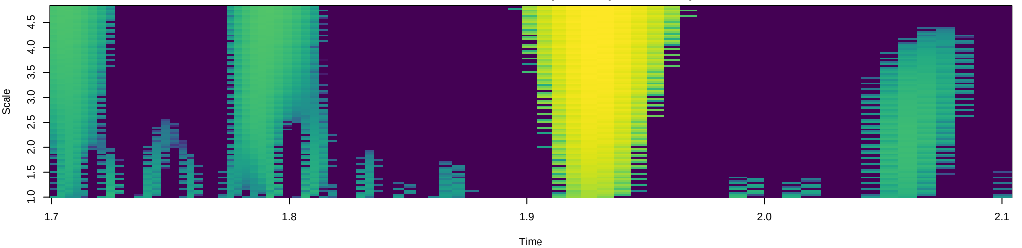
Significance Testing (Holm FWER-adjusted minimum p-values)
