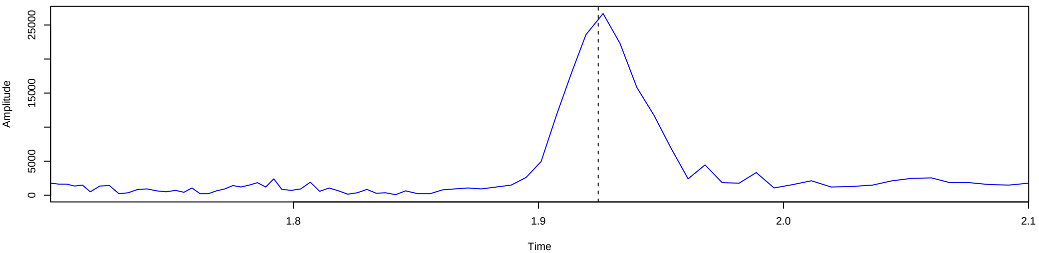
Mexican Hat Wavelet Power Spectrum (asinh scaled)
