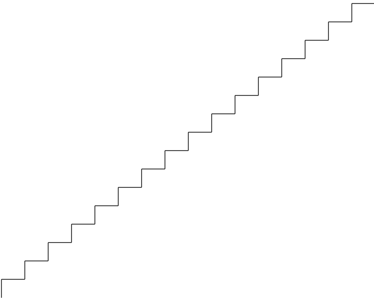
16 RISERS @ 0'-8" · 15 TREADS @ 0'-10" · TOTAL RISE 10'-6"
