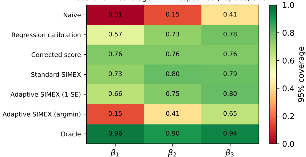
Scenario 2: coverage with misspecified (Laplace) error
