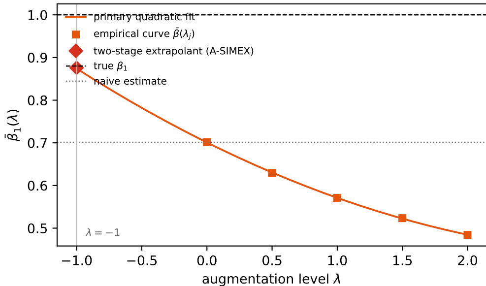
SIMEX curve diagnostic (one dataset, n = 500 , \sigma_\varepsilon^2 = 0.5 )
