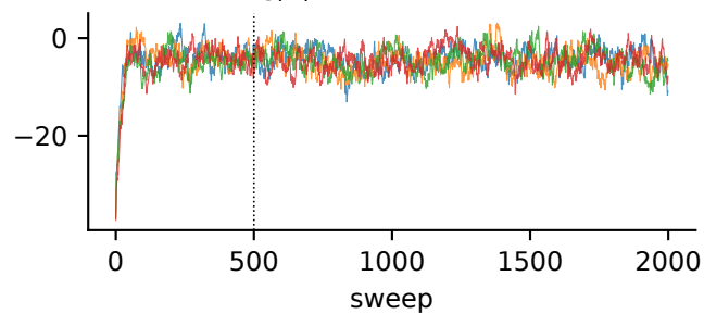
\log|\Omega| \hat{R}=1.01 , ESS=173
