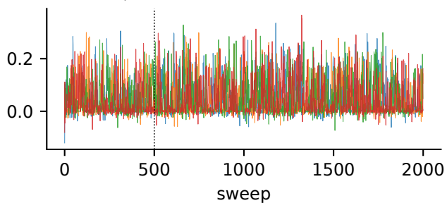
\omega_{1,2} (true 0.00) \hat{R}=1.00 , ESS=1292
