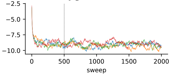
clusters per obs. \hat{R}=1.00 , ESS=890
