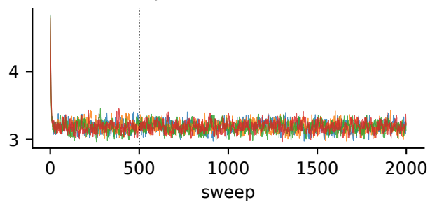
clusters per obs. \hat{R}=1.00 , ESS=890
