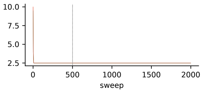
\nu : identical in all chains at 2.5
