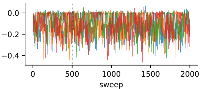
\omega_{21,32} (true -0.32) \hat{R}=1.00 , ESS=911
