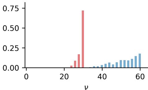
Dirichlet- t , p = 40
