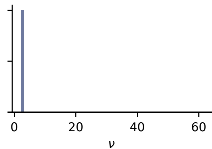
classical- t , p = 120
