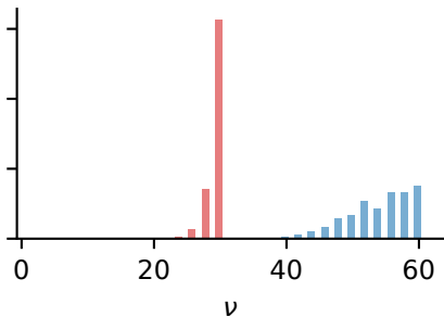
Dirichlet- t , p = 80
