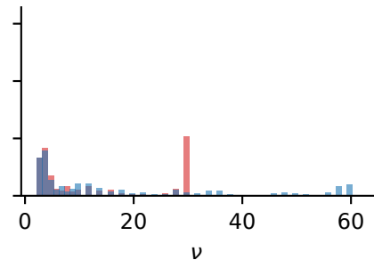
Dirichlet- t , p = 120
