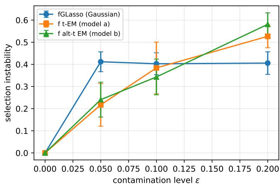
Blink artifacts, 4 of 12 channels, amplitude 6-10 sd (n=200, p=12, K=4)
