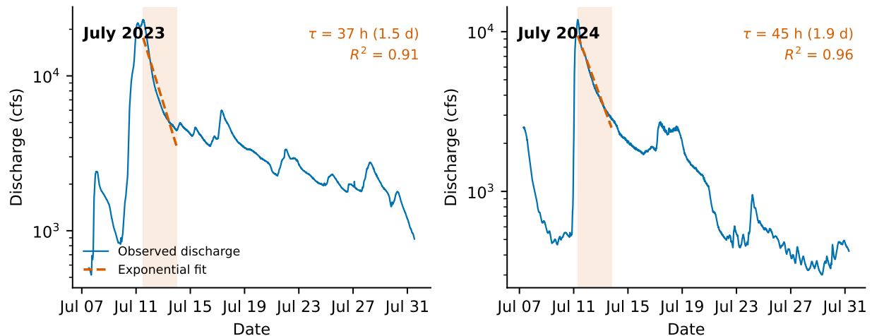
Figure 4: Recession analysis of USGS gauge 04286000 (Winooski River at Montpelier), July 2023 (left) and July 2024 (right), from 15-minute discharge records. Dashed lines show exponential fits over the shaded 60-hour windows: \tau = 37 h ( R^2 = 0.91 ) and \tau = 45 h ( R^2 = 0.96 ).
