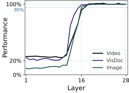
Figure 8: Qwen3-VL-2B-reranker ^{DF\uparrow} .
