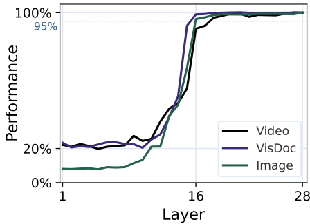
Figure 9: Qwen3-VL-2B-reranker ^{VF\uparrow} .
