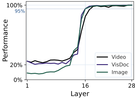
Figure 10: Qwen3-VL-2B-reranker ^{QF\uparrow} .
