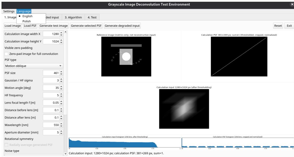
Figure 1: Main application window. Tab 1 shows the committed calculation image and PSF, their 256-bin histograms and numerical resolutions; the open Language menu documents the English/Polish GUI selector.
